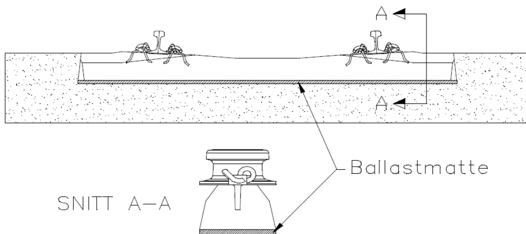
Figur 10.11 Ballastmatte under sville
