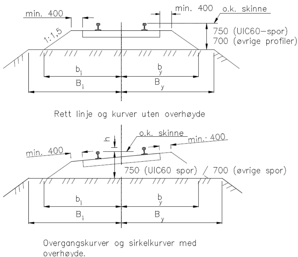
Figur 10.2 Ballastprofil for enkeltspor
