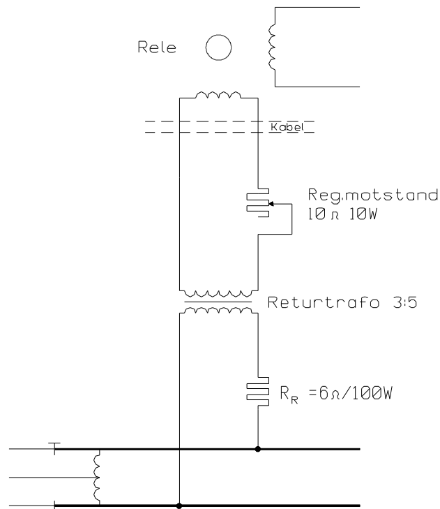
Figur 6.e.8 Retturkrets type 3.
