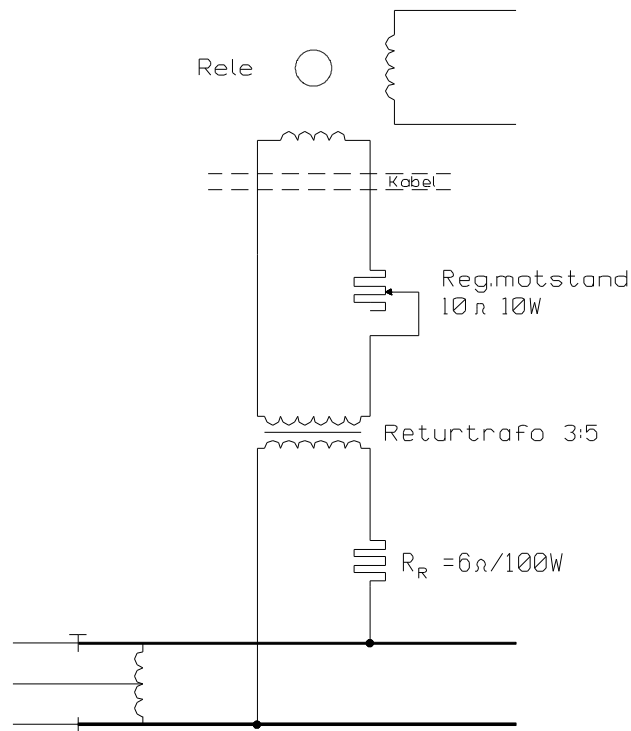
Figur 6.e.8 Retturkrets type 3.
