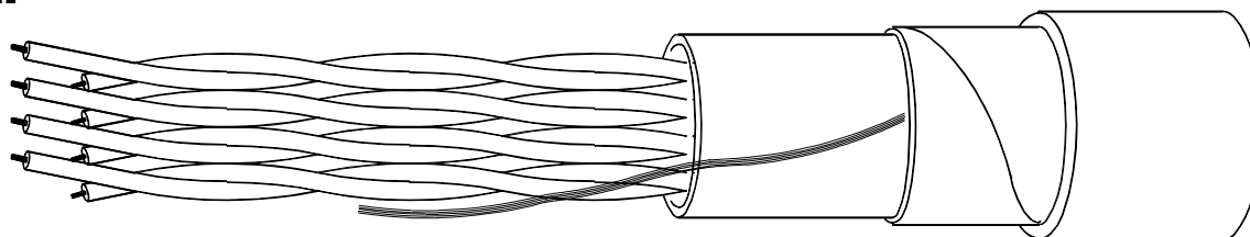
Figur 6.p.1 Signalkabel type MEBI 1kV 4x2x1,5mm 2 .
