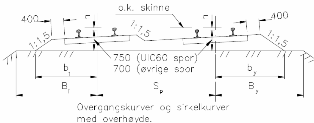
Figur 10.3 Ballastprofil for dobbeltspor
