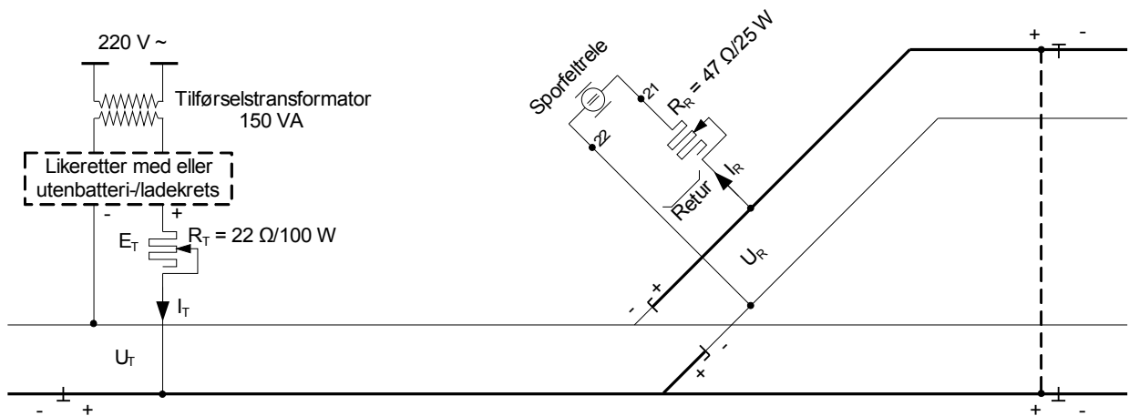
Figur 7.b.3 Likestrømsporfelt, Type 1.
