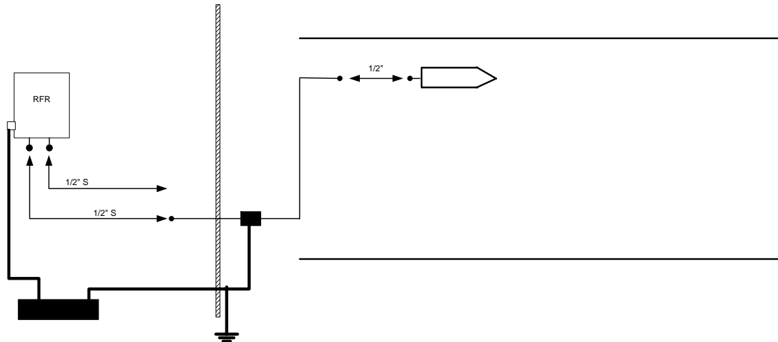
Figure 3 RF-Repeater and Tunnel Antenne
