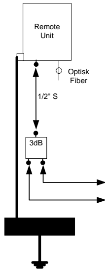
Figure 2 Grounding of Remote Unit.
