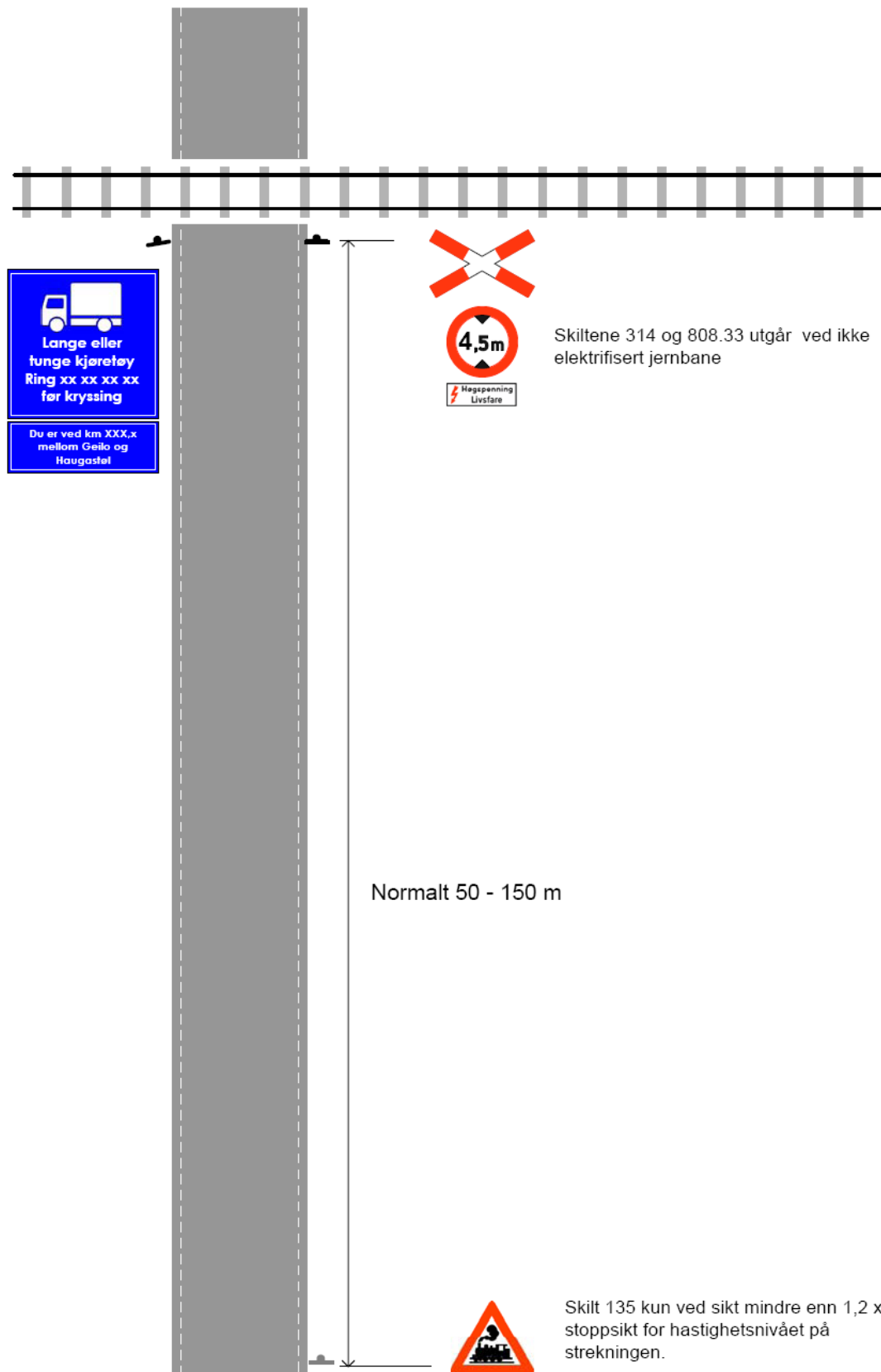
Figur 10.b.7 Planovergang type 2
