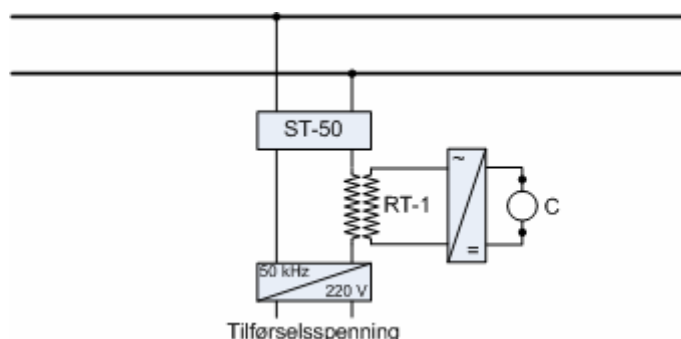
Figur 7.c.2 50 kHz sporfelt - prinsippskisse
