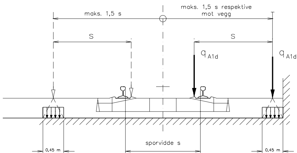
Figur 5.17 Tilfelle 1 - Ekvivalent last q_{A1d}
