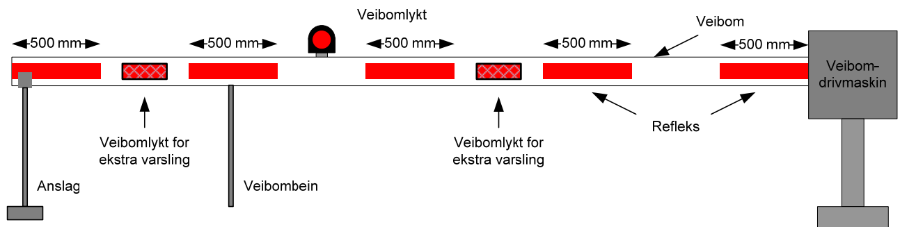
Figur 9.14 Veibom
