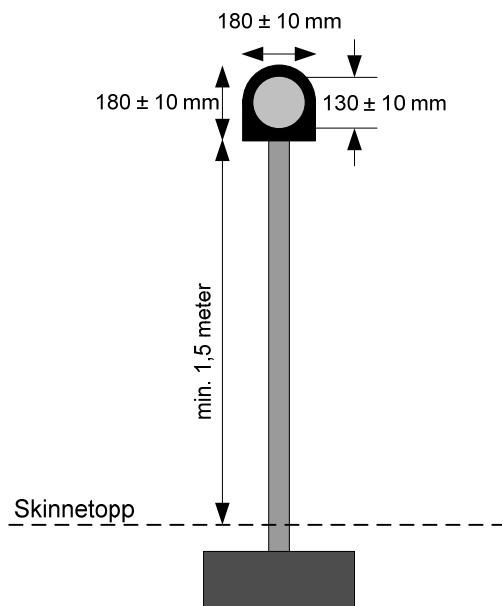
Figur 9.21 Varsellys
