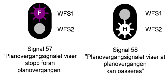
Figur 9.17 Forsignal for planovergangssignal - signalbilder
