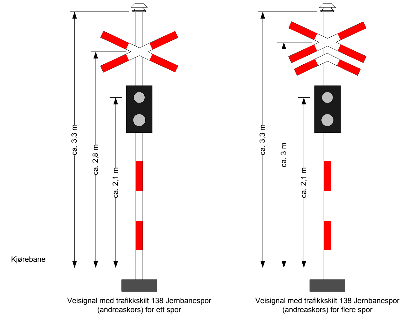
Figur 9.12 Veisignal
