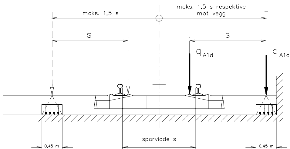
Figur 5.16 Tilfelle 1 - Ekvivalent last q_{A1d}
